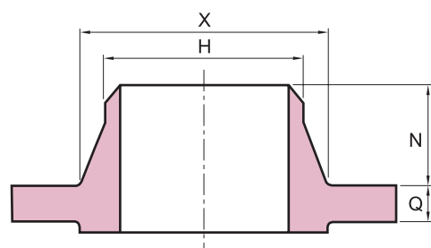
WELDING NECK
