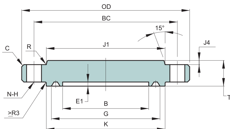
(BLIND RTJ)
